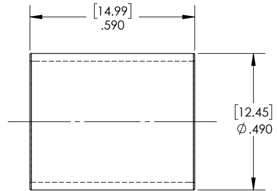
CRIMP SLEEVE
