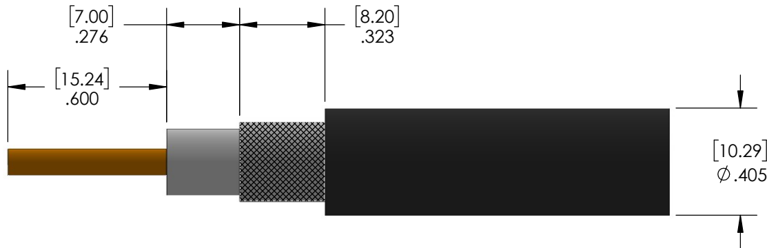
COAX STRIP DETAIL
